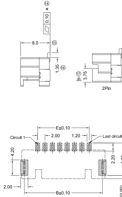
RECOMMENDED P.C.B LAYOUT (TOLERANCE:±0.05)
