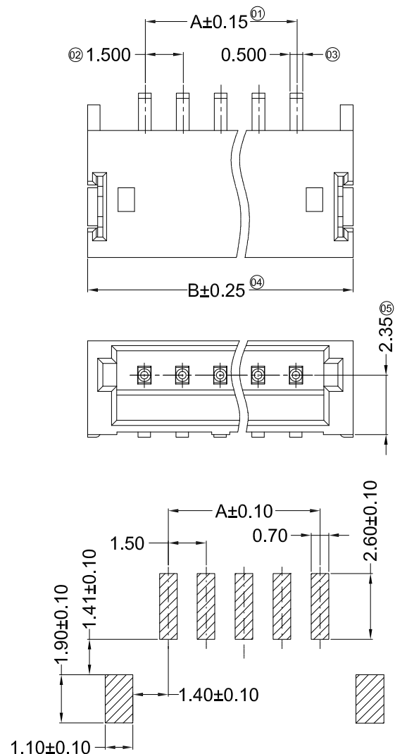
Recommended P.C.B Layout General Tolerance \pm 0.05
