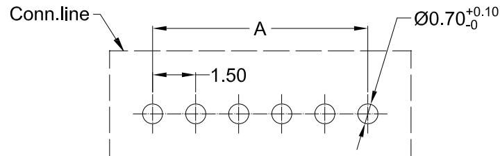
Recommended P.C.B Layout General Tolerance \pm 0.05
